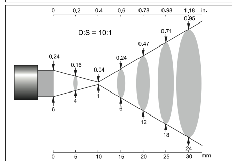
10:1 with Close Focus Accessory
