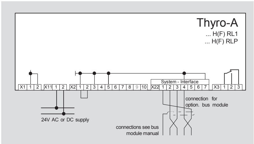
Fig. 11 Additional electronics supply and connection with optional bus module
