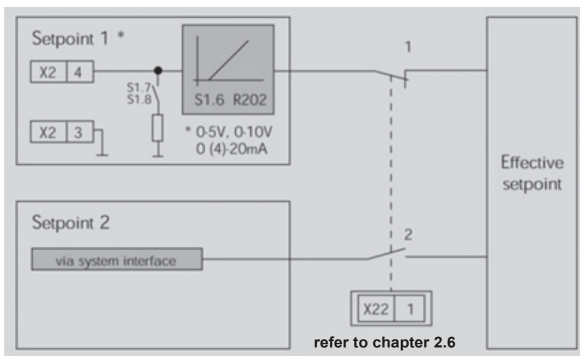
Fig. 1: Setpoint inputs and effective setpoint
