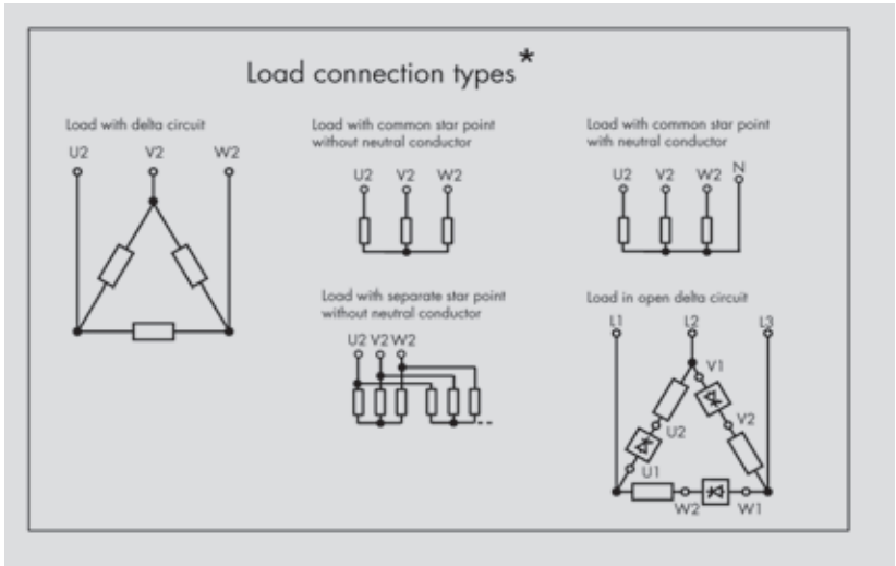
Fig. 10 Load connection types
