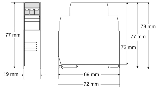
Figure 3 – Dimensions
